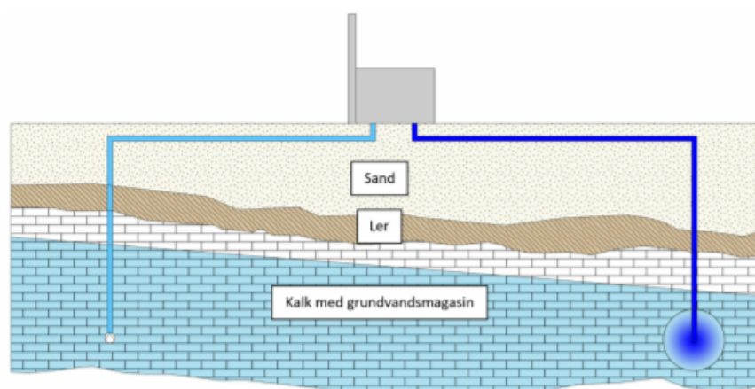
FIGUR 9: PRINCIP FOR GRUNDVANDSVARMEPUMPE (DREJEBOG FOR STORE VARMEPUMPER)
